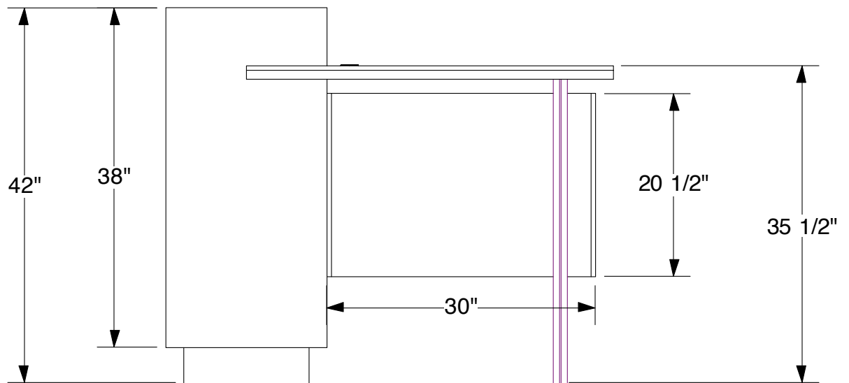
FRONT VIEW
