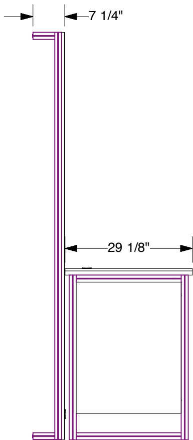
SIDE VIEW
