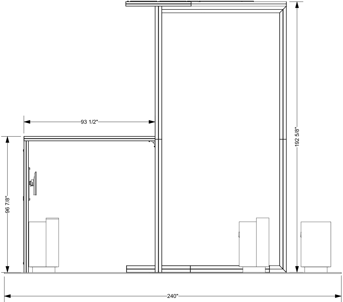
○ Left View Scale 1:35
