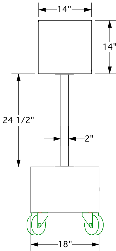
RIGHT VIEW
