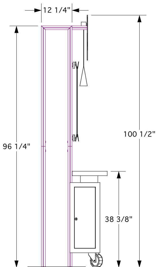
LEFT VIEW
