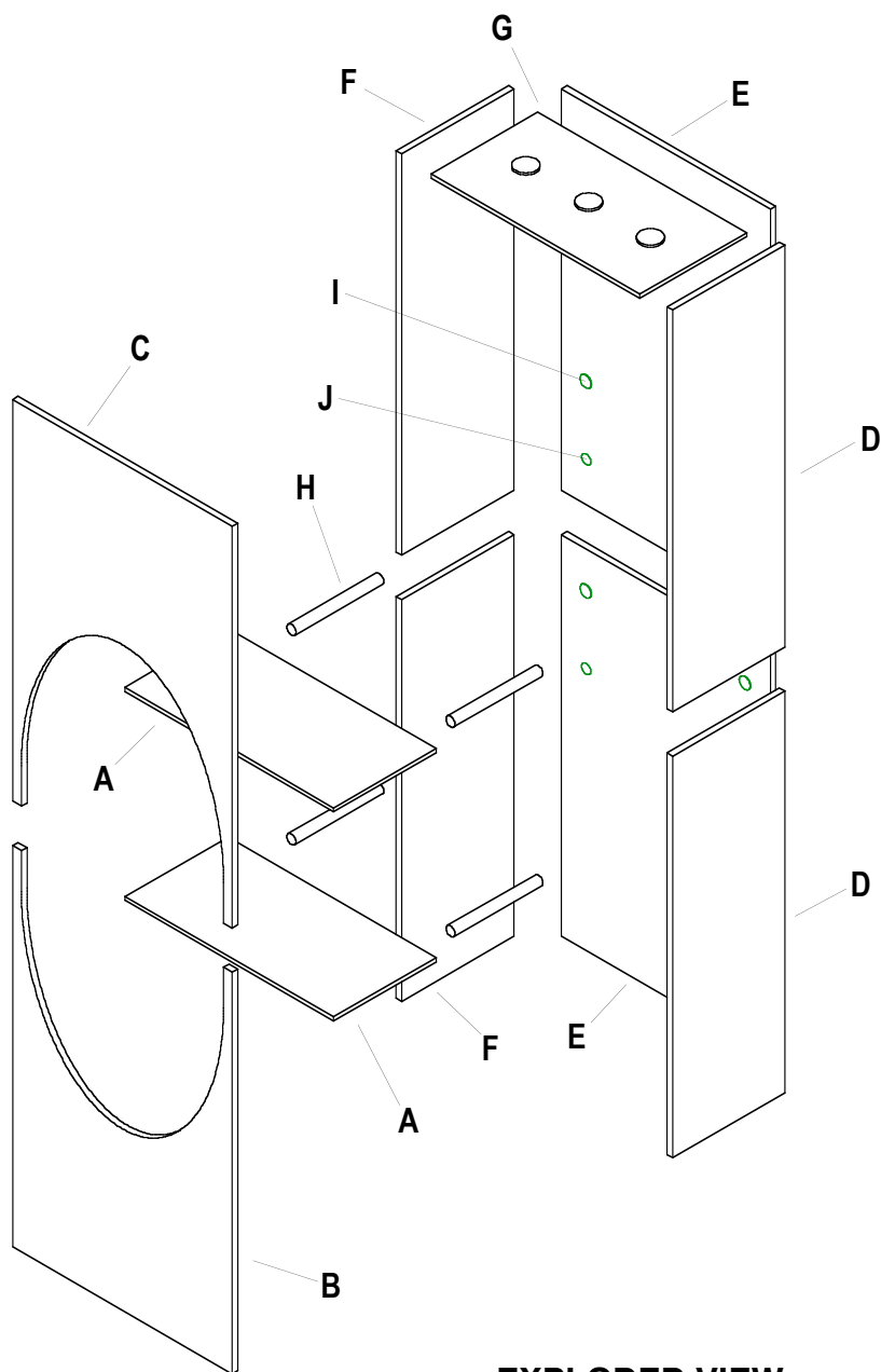
EXPLODED VIEW
