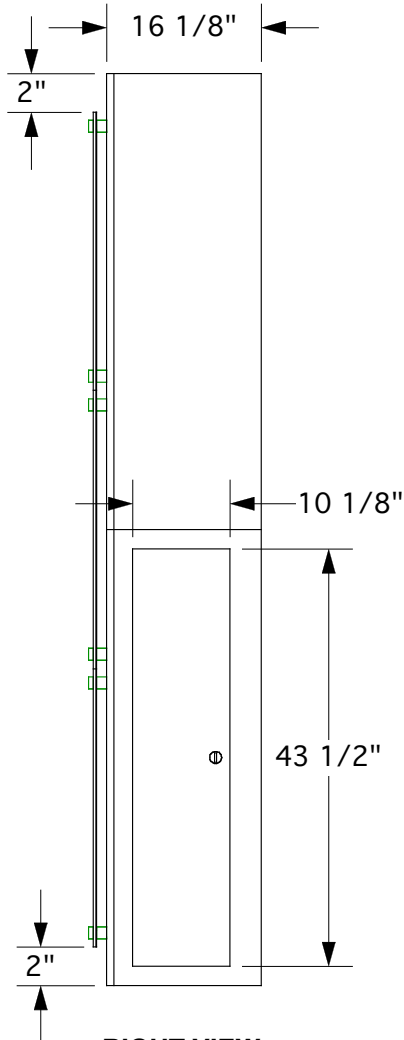
RIGHT VIEW
