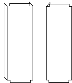
Curved Trim Set height - 25 5/8" width - 8 7/8"
