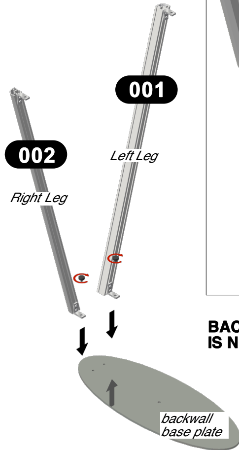
REAR VIEW
