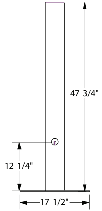
RIGHT VIEW
