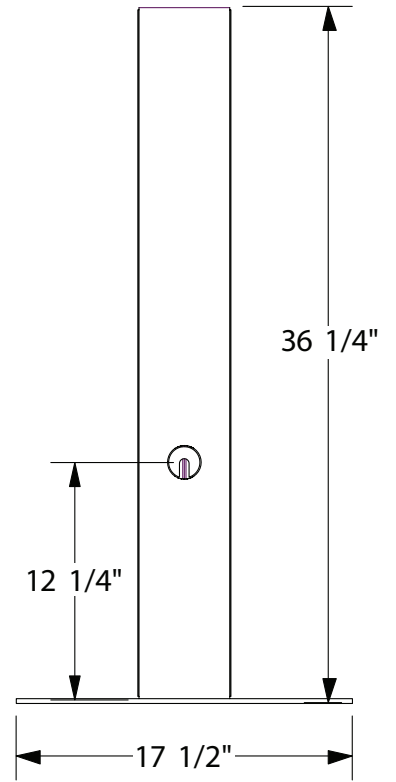
RIGHT VIEW
