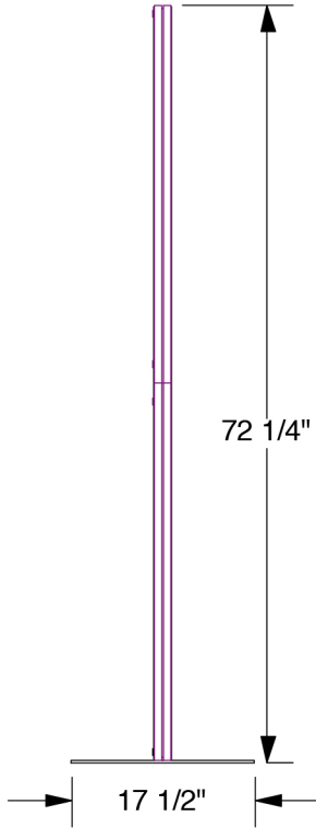
RIGHT VIEW
