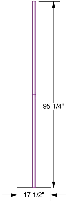
RIGHT VIEW
