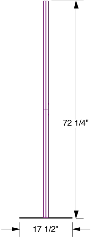
RIGHT VIEW
