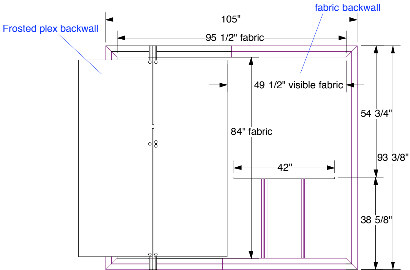
FRONT VIEW
